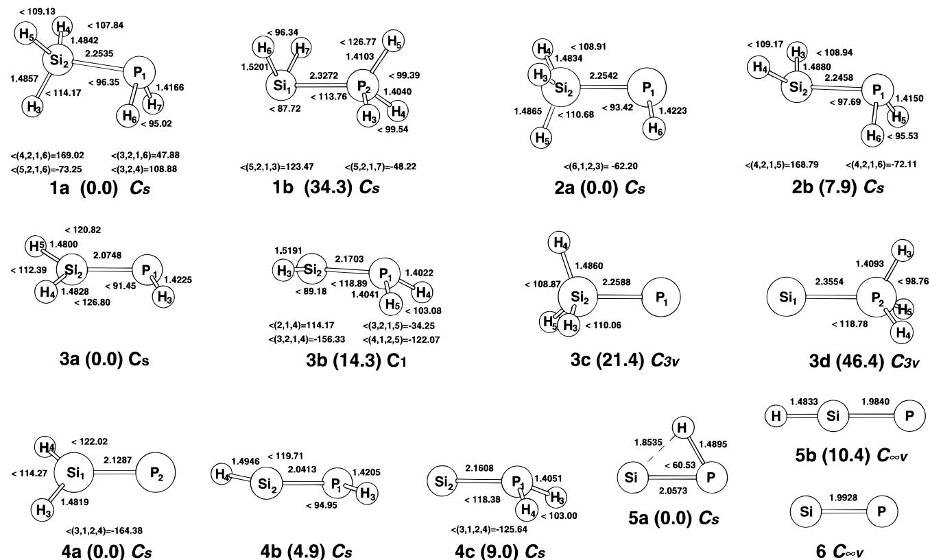
Figure 1. Equilibrium geometries for \text{SiPH}_n optimized at the MP2(full)/6-31G(d) level of theory and relative energies of isomers computed at the G2 level of theory.
